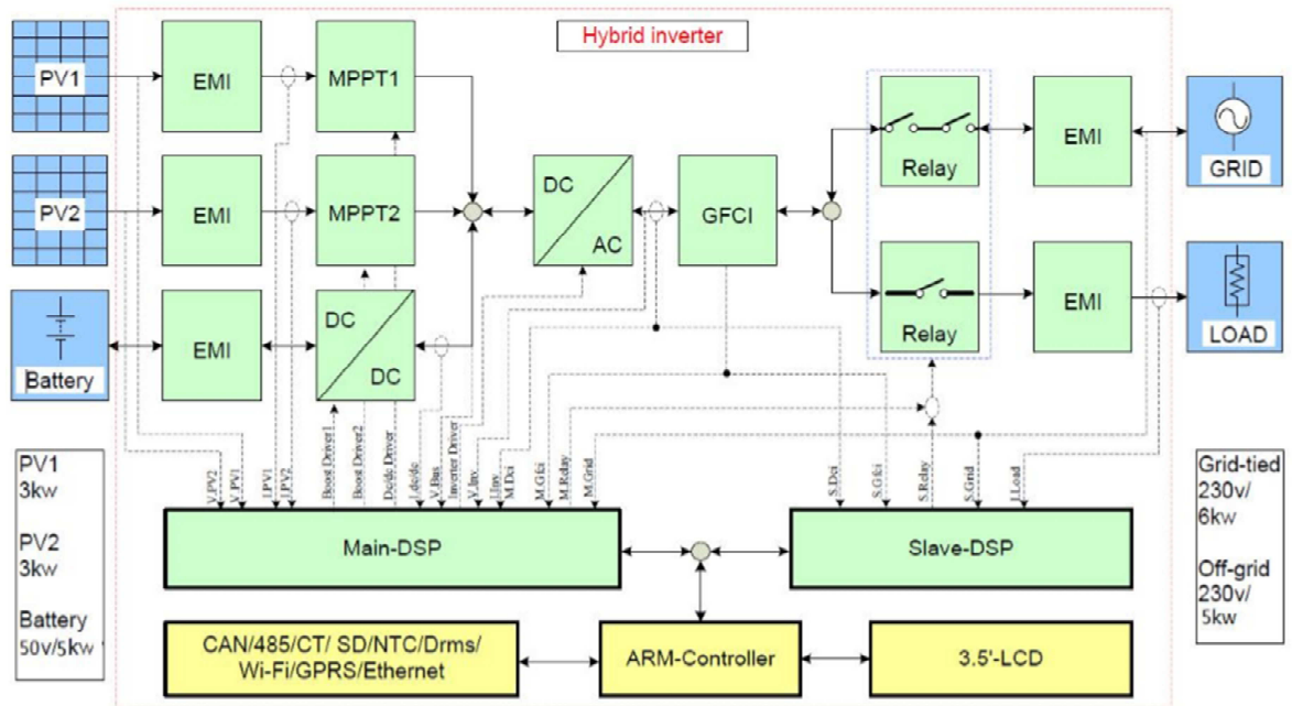
PGU Block Diagram:
